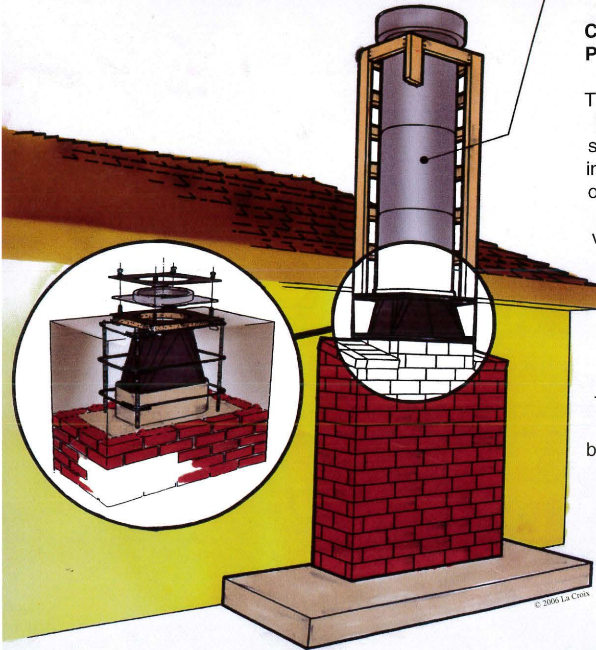
Lightweight Class-A Metal Packed Pipe Chimney System
