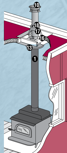
Interior installation to a stove in a mobile home.
